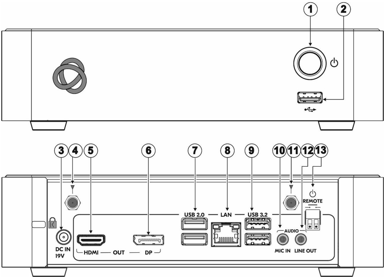
Figure 3: VIA Campus 2
