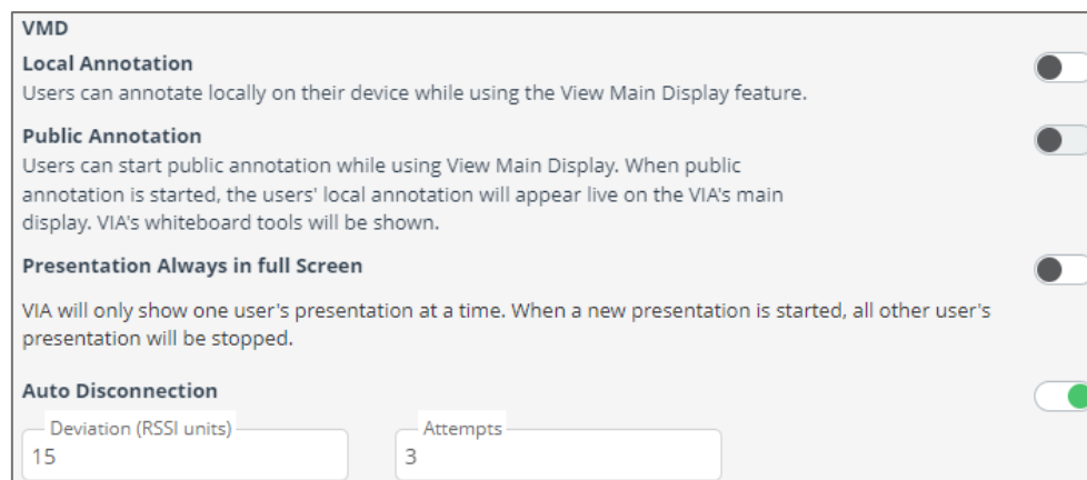
Figure 48: VMD Settings
