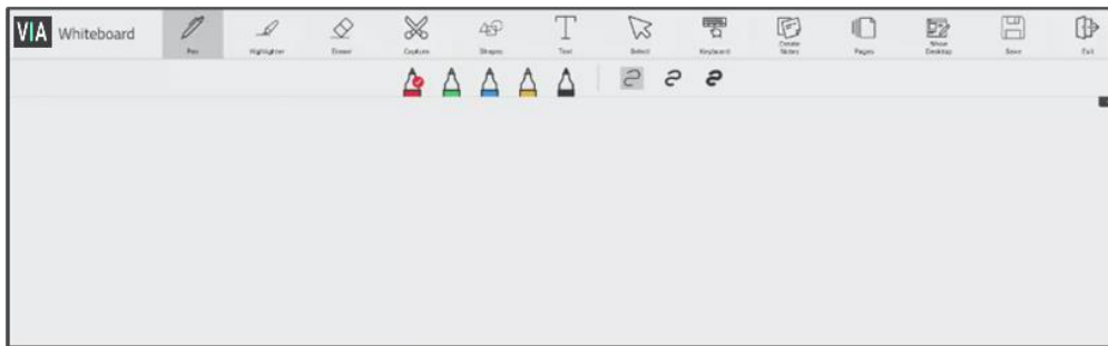
Figure 107: Whiteboard page
