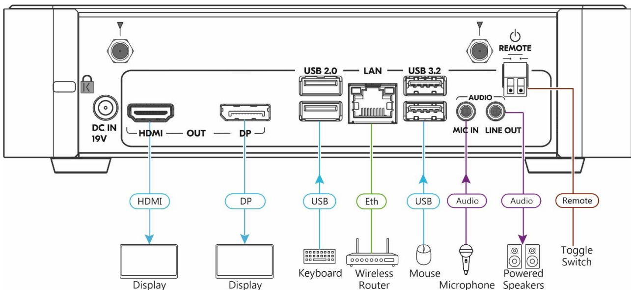
Figure 4: Connecting to the rear panel
